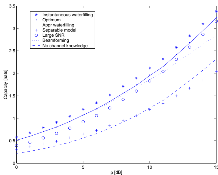
Figure 5.1: Result for N_{tx} = N_{rx} = 4 , L_p = 2 .
