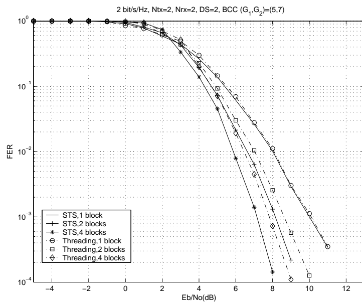
Figure 4.6: STS/Threading for (N_{tx}, N_{rx}) = (2, 2) , L = 2 , F = 1, 2, 4 .
