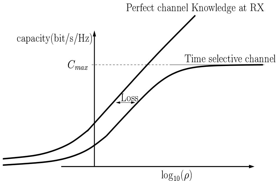
Figure 6.2: Capacity behavior of time selective channel
